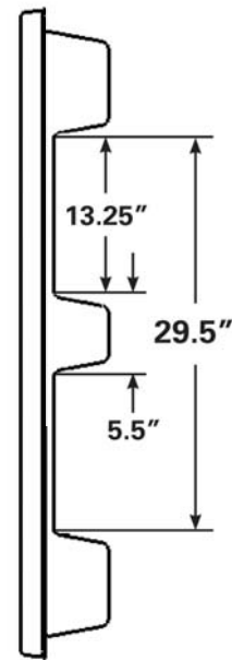
END VIEW (WIDTH)
